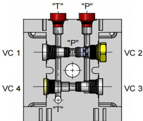
HYDRAULIC CIRCUIT 102B
