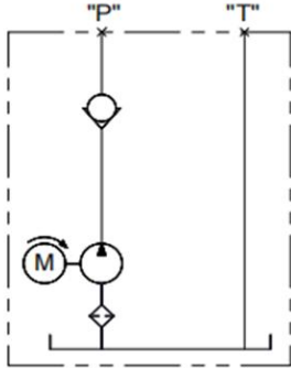
HYDRAULIC CIRCUIT 102B
