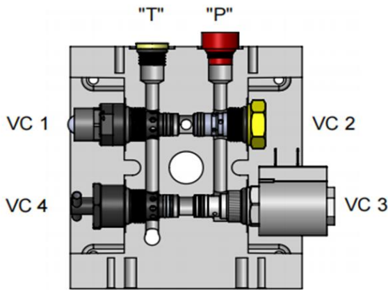
HYDRAULIC CIRCUIT 104A
