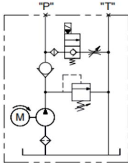
HYDRAULIC CIRCUIT 104A
