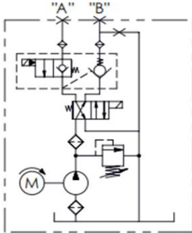
HYDRAULIC CIRCUIT 110
