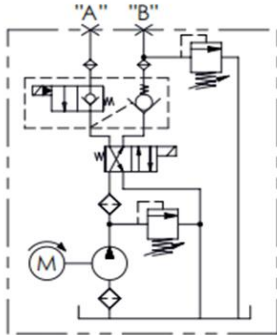
HYDRAULIC CIRCUIT 111
